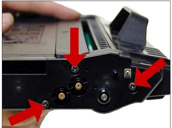
35. Clean the contacts on the left side end cap, and replace the conductive grease. Snap the end cap into place, and replace the three screws.
