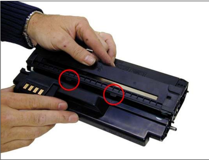
32. Slide the middle top cover/PCR assembly into place. Make sure the two middle tabs fit under the edge of the waste hopper.
