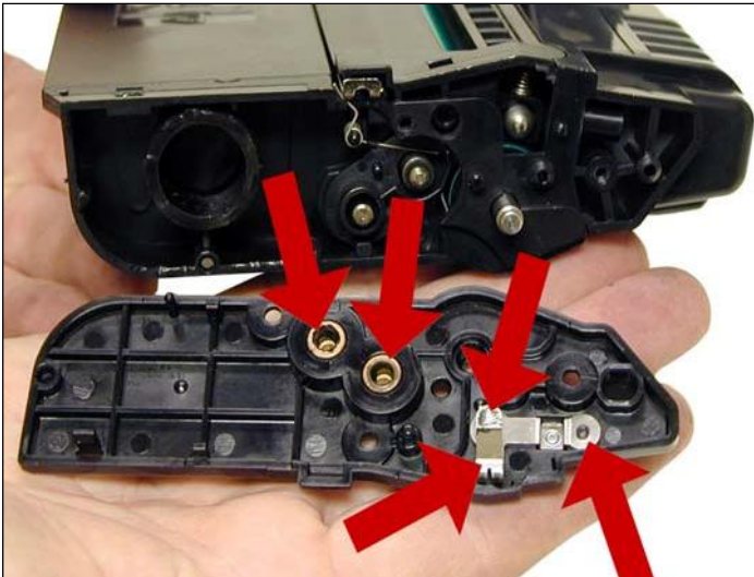
35. Clean the contacts on the left side end cap, and replace the conductive grease. Snap the end cap into place, and replace the three screws.
