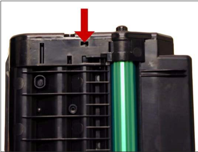
3. While still on the left end cap, locate the top and bottom tabs.
