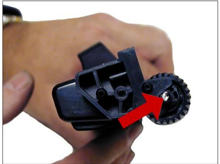
12. Remove the drum axle from the clips on both sides of the waste assembly. Remove the drum.
