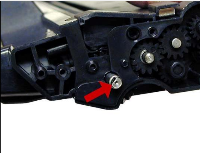
33. Take the right side end cap align the drum axle keyed end so it will fit into the keyed slot of the end cap. Snap the end cap into place.
