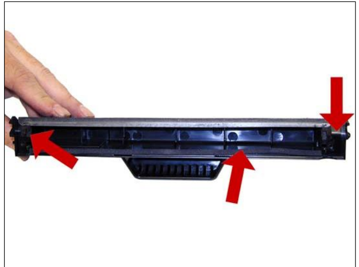
14. Remove the two screws from the doctor blade, remove the blade.
